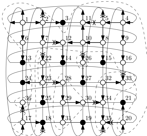
Figure 2: The partial percolation configuration after exploring all node and link events with the obtained oriented connected components. White nodes are those for which the node event N_x(Q, F) succeeds. Crossed arrows represent failed link events. The numbers near the nodes indicate the order in which the node events are tested.
