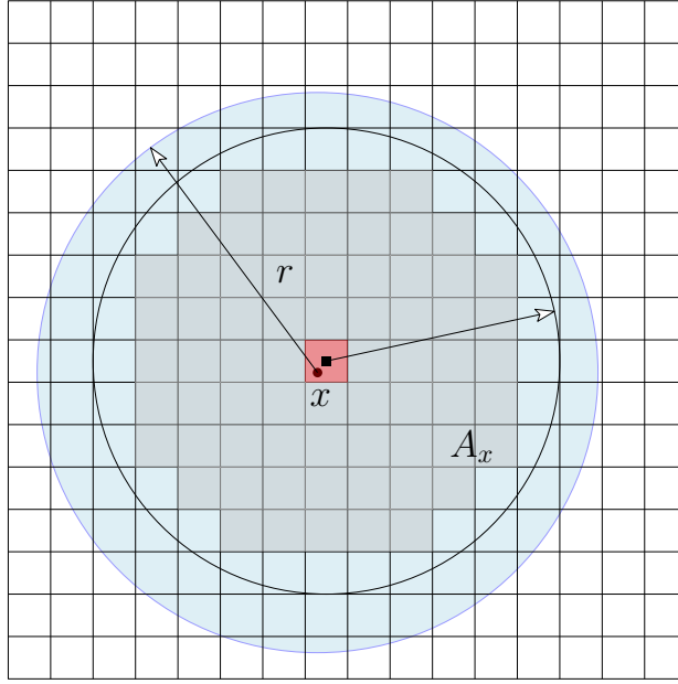
Figure 3: Any circle of radius r_n centered at x fully contains A_x which is a copy of a fixed collection of boxes.
