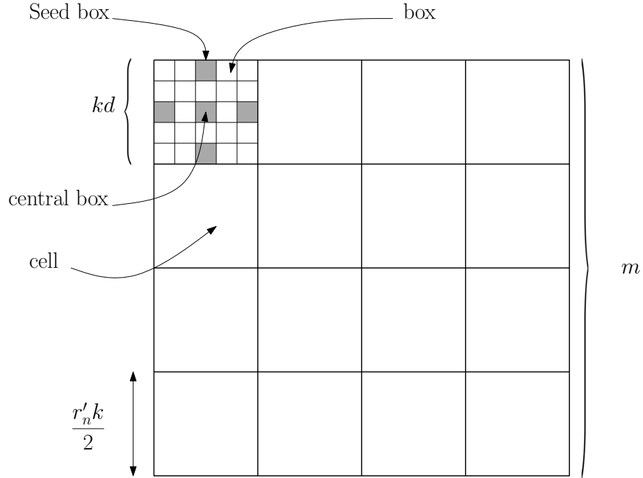
Figure 1: The different levels of discretization of the torus [0, 1]^2 are shown here with k = 5 , d = 1 , and m = 4 . The torus is sub-divided into m^2 congruent squares, called cells, and each cell is further divided into k^2 d^2 small squares, called boxes. The central box and the seed boxes of one of the cells are marked.
