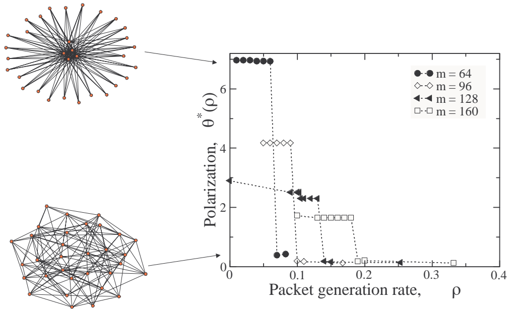
Figure 1: Polarization of the optimal structure as a function of \rho , for networks of size n = 32 and different number of links m = 64, 96, 128, 160 . The star-like configuration (top left) is optimal for low \rho , while an homogeneous configuration (bottom left) is optimal for high \rho .
