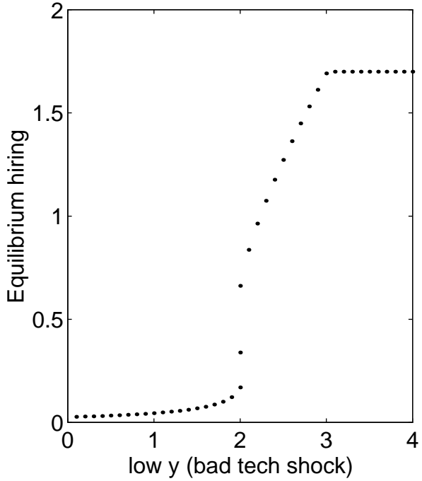
Fig.15: Equilibrium correspondence
