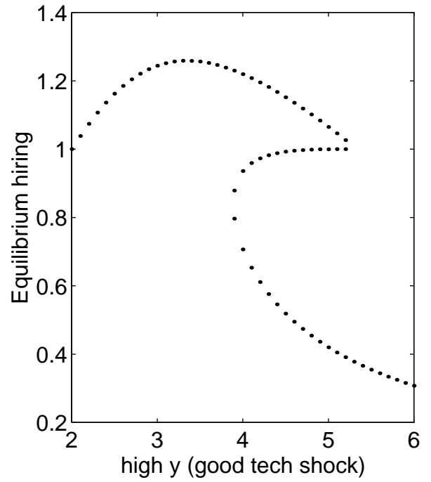
Fig.8: Equilibrium correspondence
