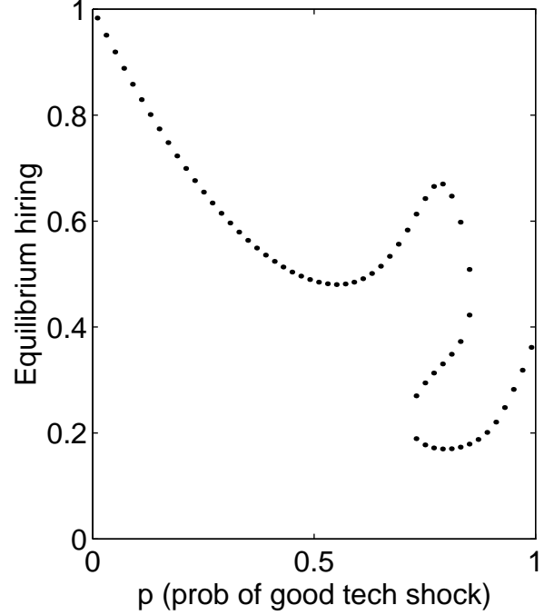
Fig.14: Equilibrium correspondence
