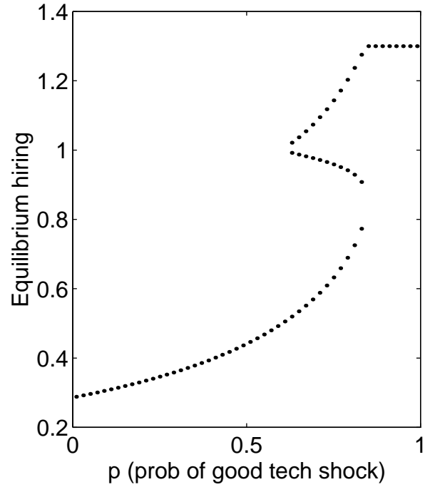
Fig.6: Equilibrium correspondence
