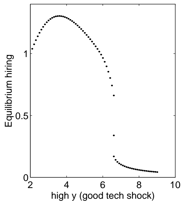
Fig.16: Equilibrium correspondence
