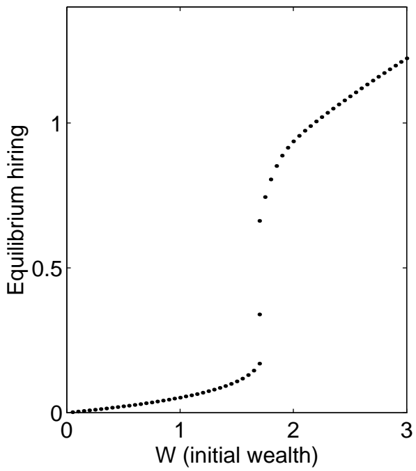
Fig.13: Equilibrium correspondence
