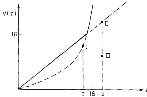
FIG. 4. V(z) = \text{Max}_{x_1 + x_2 = z} x_1 + \frac{1}{16}(x_2)^2 ; a = 8(2\sqrt{6} - 3) ; b = \frac{120}{7} .
