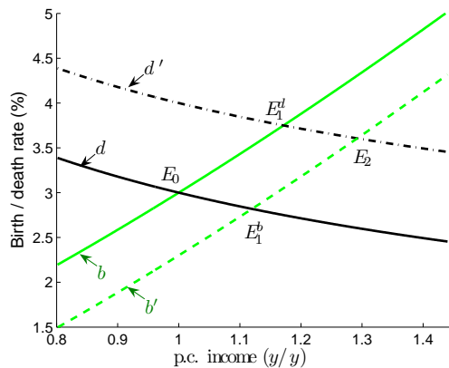
Figure 1: Long-run equilibria
